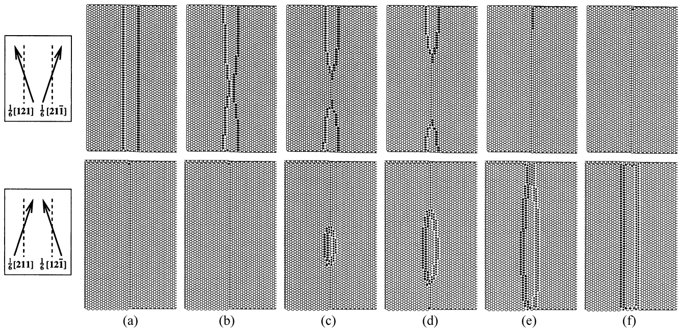
FIG. 1. Minimum energy transition path for cross slip of a screw dislocation. Top: primary glide plane ( \bar{1}\bar{1}1 ). Bottom: cross-slip plane ( \bar{1}1\bar{1} ). The Burgers vectors in each glide plane are indicated to the left. (a) Starting configuration with parallel Shockley partials in the primary glide plane. (b) Recombination into a constriction entirely in the primary plane. (c) Redissociation in the cross-slip plane. The upper constriction is screwlike, and the lower is edgelike. (d) Transition state with half of the dislocation in either glide plane. (e) Single plane constriction entirely in the cross-slip plane. (f) The cross-slip process is complete, with parallel Shockley partials in the cross-slip plane.
