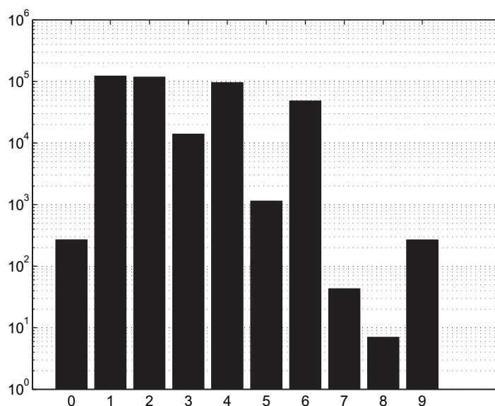
Figure 14. Histogram showing the distribution of atoms being displaced by more than 0.5 \text{ \AA} . The analysis extends over the first 400 000 transitions. When the four most abundant transition types are accounted for (1, 2, 4 and 6 atoms), only 4% of the transitions remains. A transition involving either four or six atoms occurs almost as frequently as a transition involving only a single atom.
